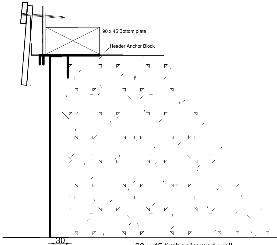
90 x 45 timber framed wall Header Anchor Block XPS foam
