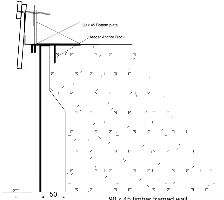
90 x 45 timber framed wall Header Anchor Block EPS foam
