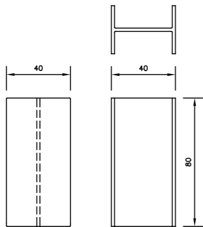
InsulAPE Joiner Square-Top APE-30-300-CI-SQ (300mm) Pre-Install
